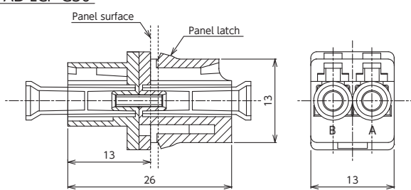
For LCF connector
