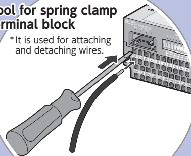
Example used a tool for spring clamp terminal block
