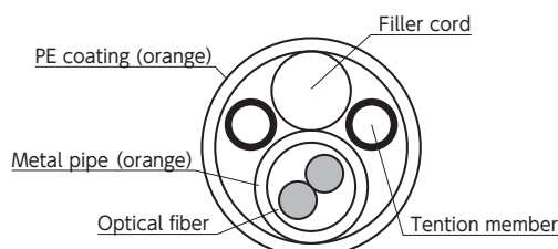
Structure for 2-core type
