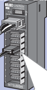
Open sensor connector Type A, M
