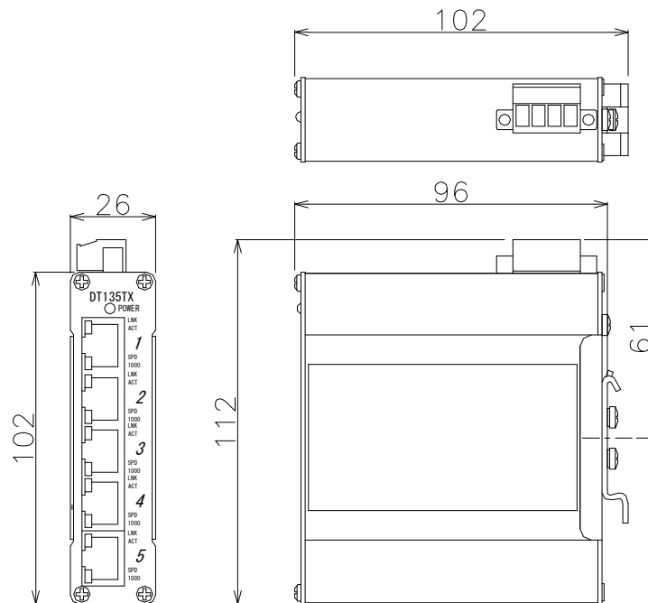
Figure 6.1 External dimensions
