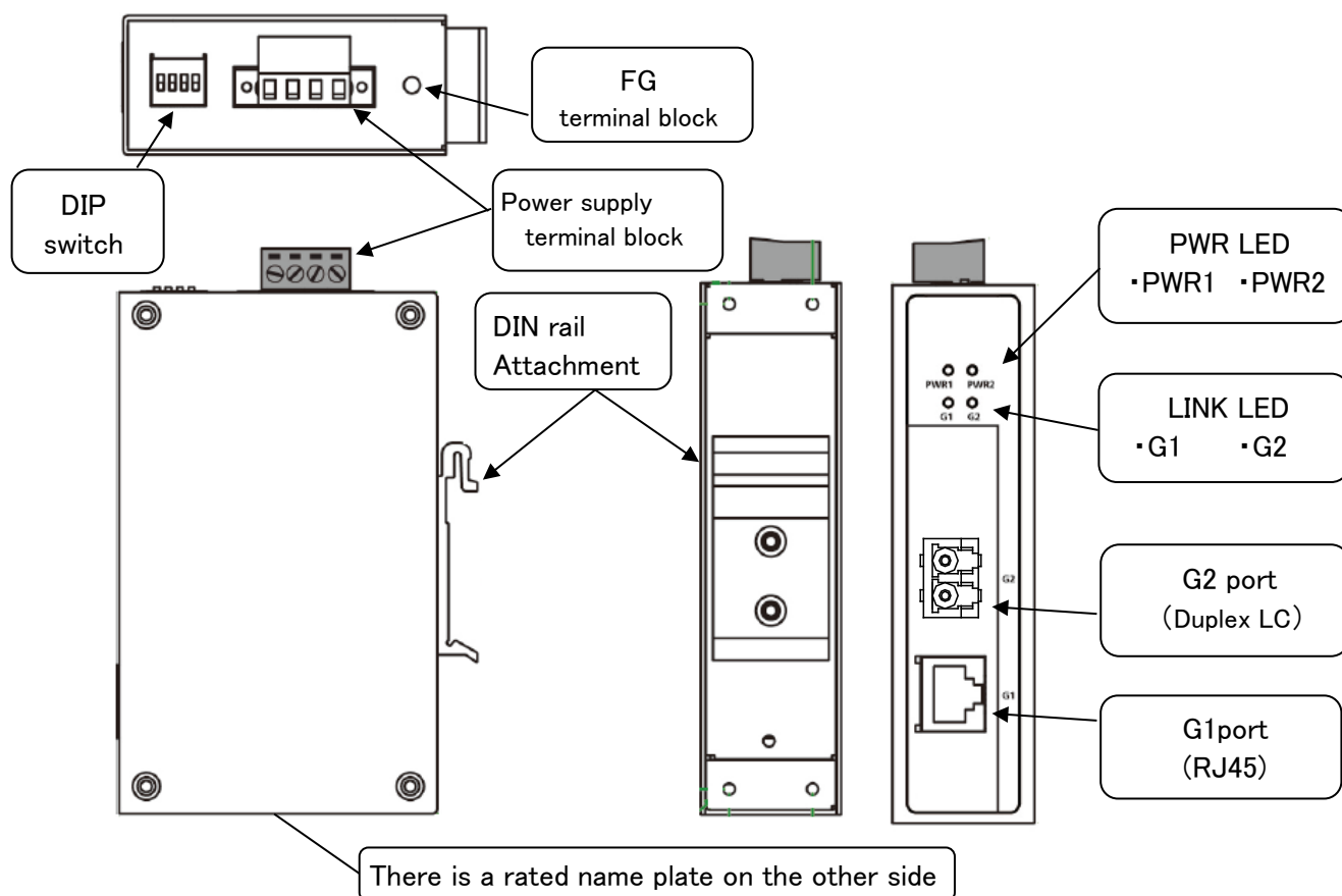
Figure 4.1 Names of parts
