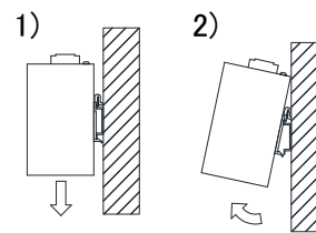
Figure 5.4 Removed method
