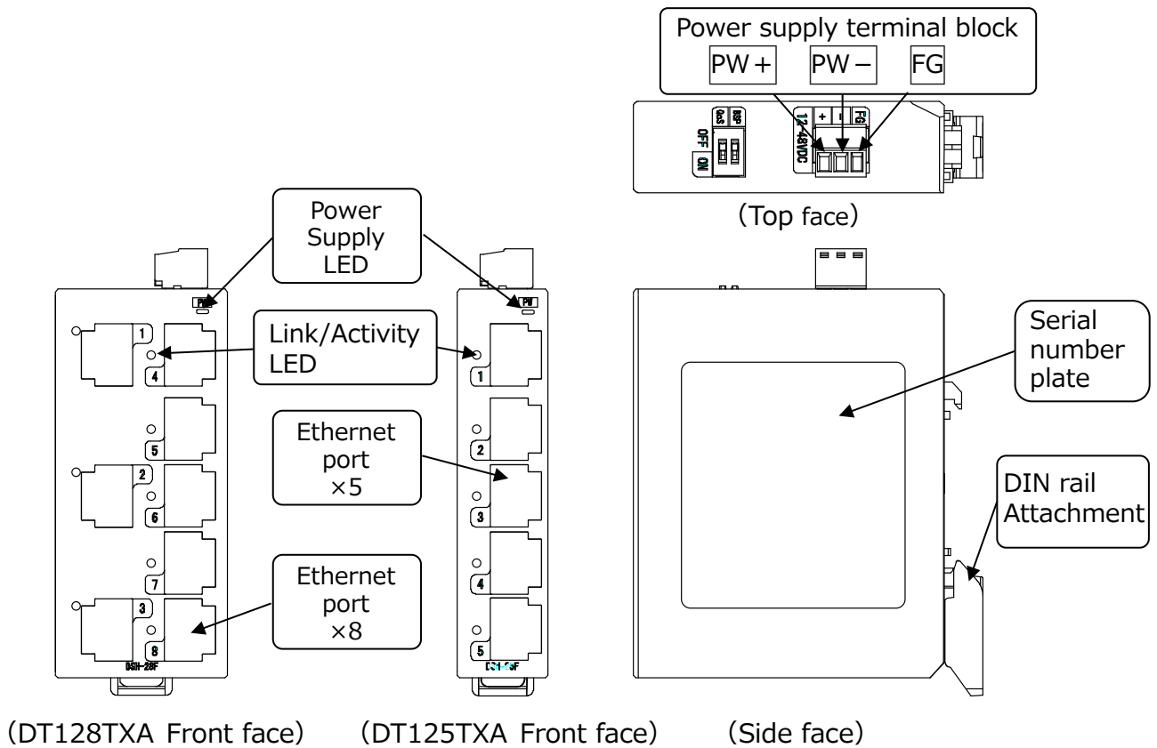
Figure 4.1 Names of parts
