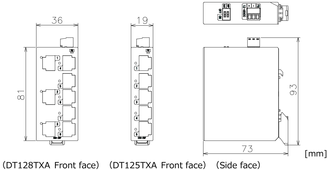
Figure 6.1 External dimensions
