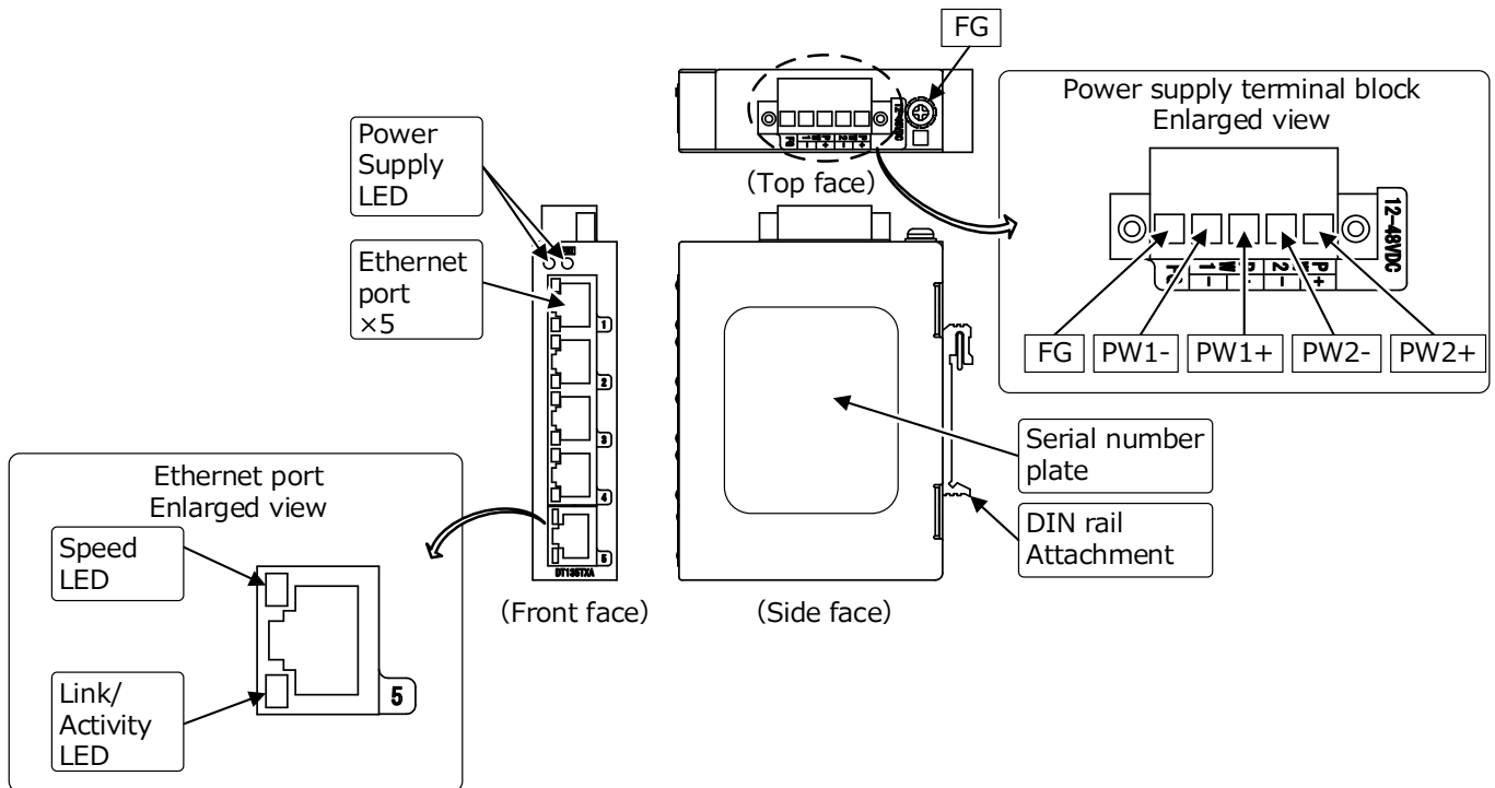
Figure 4.1 Names of parts
