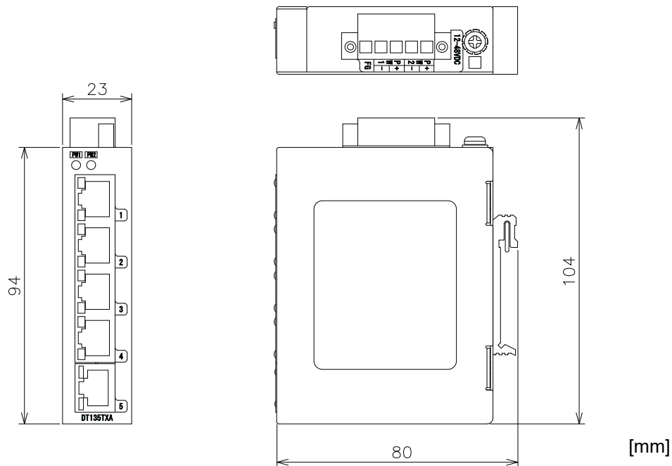
Figure 6.1 External dimensions
